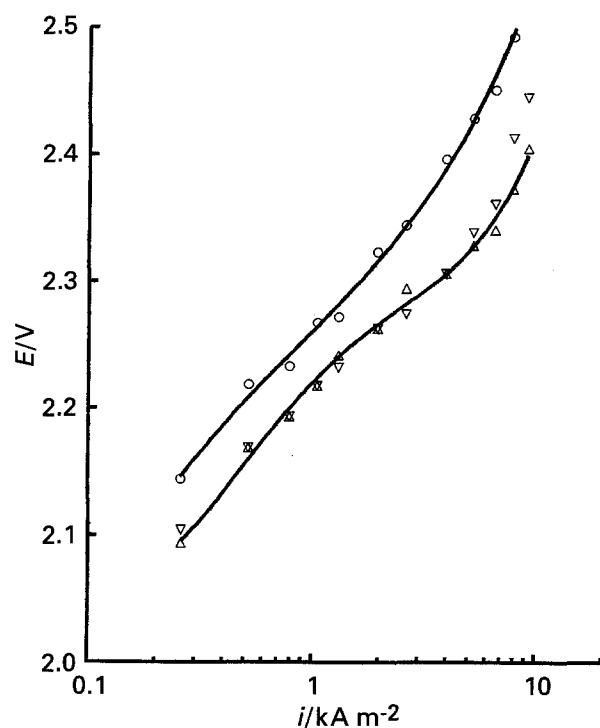
Fig. 4. Galvanostatic polarization curves for a platinum anode in a 3.76 \text{ m NaClO}_3 + 1.64 \text{ m NaClO}_4 solution at various solution flow rates u_s and at 50°C. Key: (○) u_s = 0.06 \text{ m s}^{-1} , (▽) u_s = 0.24 \text{ m s}^{-1} and (△) u_s = 0.33 \text{ m s}^{-1} .
