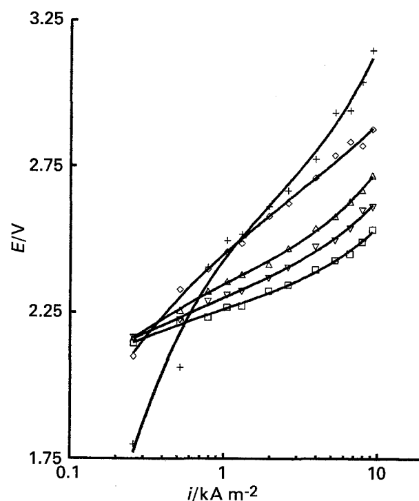
Fig. 5. Galvanostatic polarization curves for a platinum anode in solutions containing 1.64 \text{ m NaClO}_4 and various concentrations of \text{NaClO}_3 , at a solution-flow rate of 0.06 \text{ m s}^{-1} and at 50°C. \text{NaClO}_3 concentrations: Key: (+) 0.038 \text{ m} , (◇) 0.47 \text{ m} , (△) 0.94 \text{ m} , (▽) 2.35 \text{ m} and (□) 3.76 \text{ m} .
