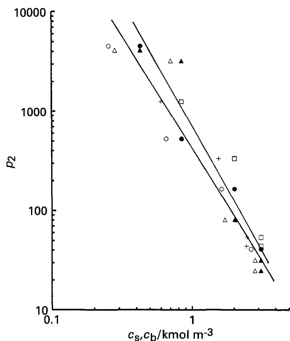
Fig. 13. Parameter p_2 against c_s and c_b on a double logarithmic scale for electrolyses at a platinum anode in solution containing 1.64 M NaClO 4 and various NaClO 3 concentrations at 50°C and a solution flow rate of 0.06 m s -1 , where p_2 = 10^{-2} \{ [(4\Gamma_{O_2}/\Gamma_{ClO_4}) + 1]^2 - 1 \} \exp(-(\alpha_a - \alpha_g)f(E - 2.0)) at c_b and at i = 0.79 (▲), 1.05 (●) and 1.31 kA m -2 (□), for mechanism IV.
