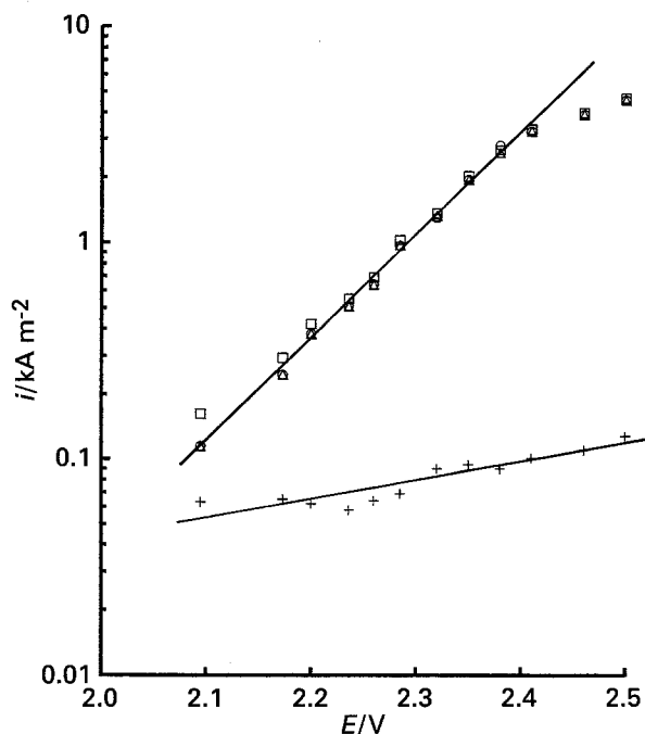
Fig. 10. Electrode potential plotted against \ln i_a for an electrolysis at a platinum anode in a solution containing 3.76\text{ m NaClO}_3 + 1.64\text{ m NaClO}_4 and at 50^\circ\text{C} and a solution flow of 0.33\text{ m s}^{-1} , where i_a = i_{\text{O}_2} ( + ), i - 0.5 i_{\text{ClO}_4} - 0.75 i_{\text{O}_2} ( \Delta ), 0.5 i_{\text{ClO}_4} + 0.25 i_{\text{O}_2} ( \circ ) and i - 0.5 i_{\text{ClO}_4} ( \square ) for mechanism I, II, III and IV, respectively.
