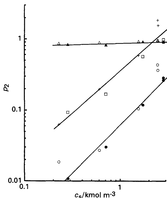
Fig. 12. Parameter p_2 against c_s on a double logarithmic scale for electrolyses at a platinum anode in a solution containing 1.64 M NaClO_4 and various NaClO_3 concentrations, and at 50°C and a solution flow rate of 0.06 \text{ ms}^{-1} , where p_2 is (\Gamma_{ClO_4}/\Gamma_{O_2}) \exp \{-(\alpha_b - \alpha_a)f(E - 2.0)\} at i = 0.79 ( \square ) and 1.31 \text{ kA m}^{-2} (+), [2\Gamma_{ClO_4}/(2\Gamma_{ClO_4} + \Gamma_{O_2})] \exp \{-(\alpha_b - \alpha_a)f(E - 2.0)\} at i = 0.79 ( \Delta ) and 1.31 \text{ kA m}^{-2} ( \circ ), (\Gamma_{ClO_4}/\Gamma_{O_2}) \exp \{-(\alpha_g - \alpha_e)f(E - 2.0)\} at i = 0.79 ( \bullet ) and 1.31 \text{ kA m}^{-2} ( \circ ), for the mechanisms I-III.
