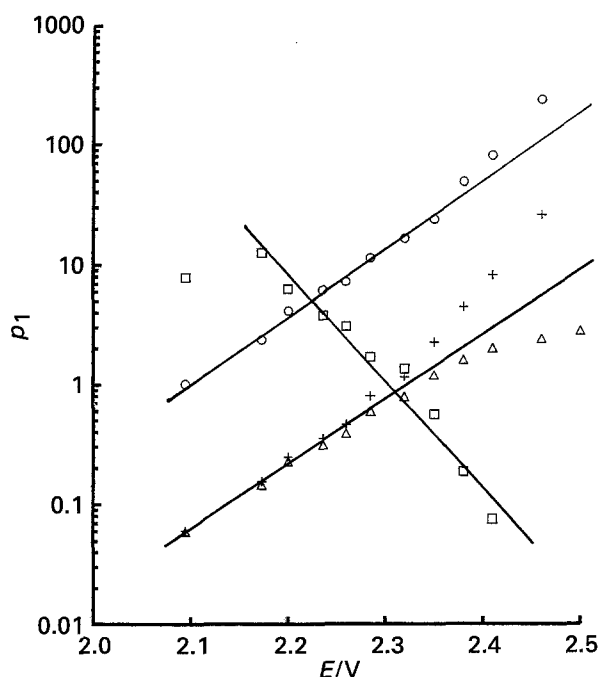
Fig. 11. Electrode potential against \ln p_1 for electrolysis at a platinum anode in solution containing 3.76 M NaClO_3 + 1.64 M NaClO_4 at 50°C and a solution flow of 0.33 \text{ ms}^{-1} , where p_1 = i_{ClO_4}/2c_s (+) and i_{ClO_4}/2c_b ( \Delta ) for mechanisms I and II, p = i_{ClO_4}/c_s i_{O_2} for mechanism III ( \circ ), and c_s^2 \{[(4i_{O_2}/i_{ClO_4}) + 1]^2 - 1\} for mechanism IV ( \square ) and i_{O_2} and i_{ClO_4} are given in \text{kA m}^{-2} and c_s and c_b in \text{kmol m}^{-3} .
