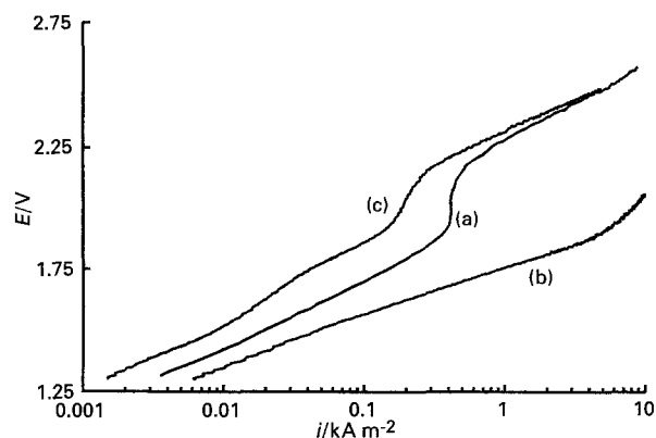
Fig. 3. Potentiodynamic polarization curves for a platinum anode in various solutions and at 50°C. Potential scan rate is 5 \text{ mV s}^{-1} . (a) 3.76 \text{ m NaClO}_3 , (b) 1.64 \text{ m NaClO}_4 and (c) 3.76 \text{ m NaClO}_3 + 1.64 \text{ m NaClO}_4 .
