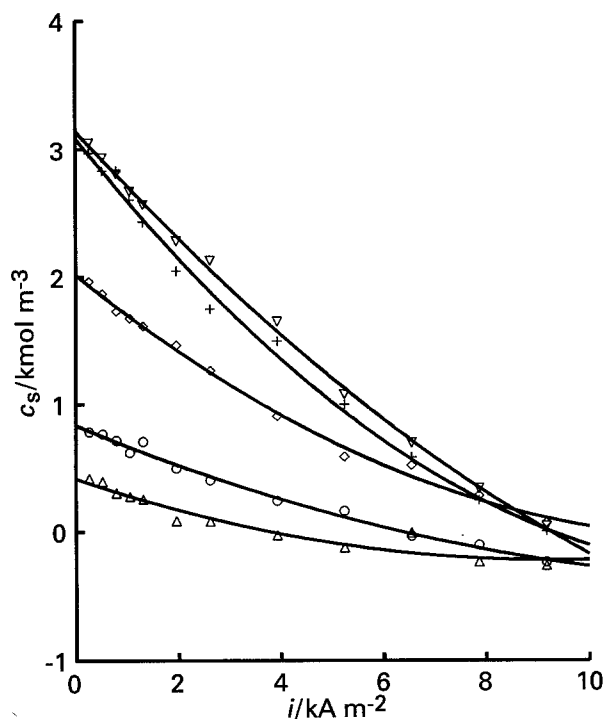
Fig. 9. Chlorate concentration at platinum anode surface as a function of current density for electrolyses in solutions containing 1.64\text{ m NaClO}_4 and various concentrations of \text{NaClO}_3 : ( \Delta ) 0.47\text{ m} , ( \circ ) 0.94\text{ m} , ( \diamond ) 2.35\text{ m} and ( + ) 3.76\text{ m NaClO}_3 at a solution flow rate of 0.06\text{ m s}^{-1} and in 1.64\text{ m NaClO}_4 + 3.76\text{ m NaClO}_3 ( \nabla ) at a solution flow rate of 0.33\text{ m s}^{-1} . Temperature: 50^\circ\text{C} .
