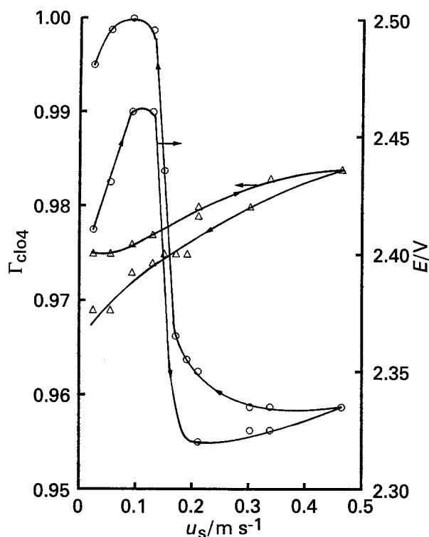
Fig. 7. Perchlorate current efficiency ( \triangle ) and electrode potential ( \circ ) as a function of solution flow rate for a platinum anode in a 4.69\text{ m NaClO}_3 solution at a current density of 6.55\text{ kA m}^{-2} and at 50^\circ\text{C} . The arrows on the curves indicate the direction of the change in the flow rate of solution.
