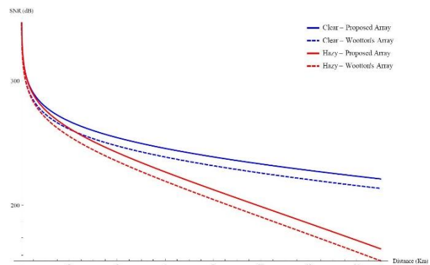
Fig. 14 Signal-to-Noise Ratio for the proposed optical array in clear and hazy atmospheric conditions.
